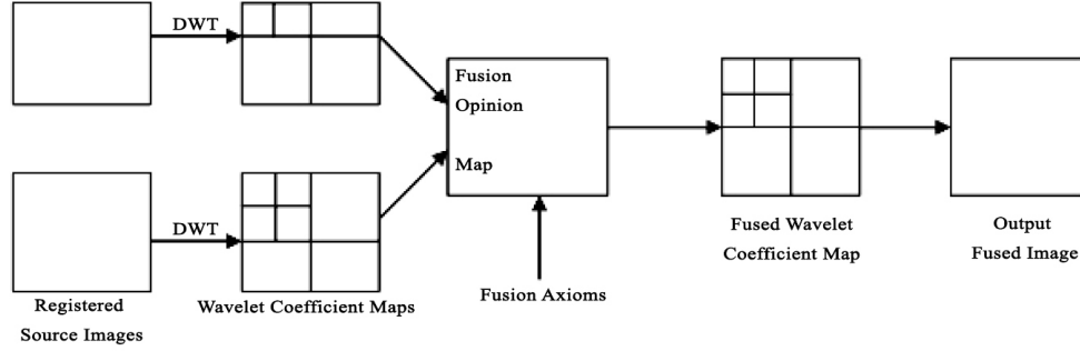
Figure 1: The generic structure for wavelet transform based image fusion
