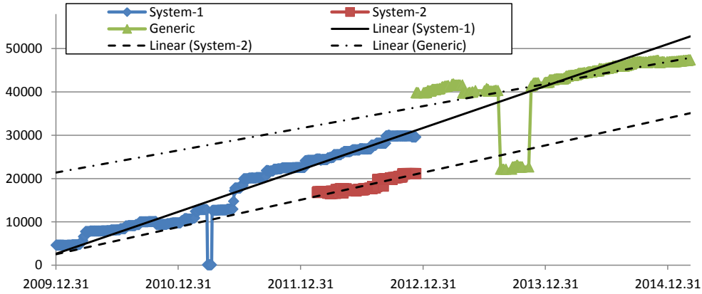
Figure 2: Number of magic string issues and its linear approximations.
