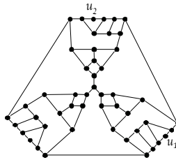
Figure 2: CPB3C non-Hamiltonian graph G - x
