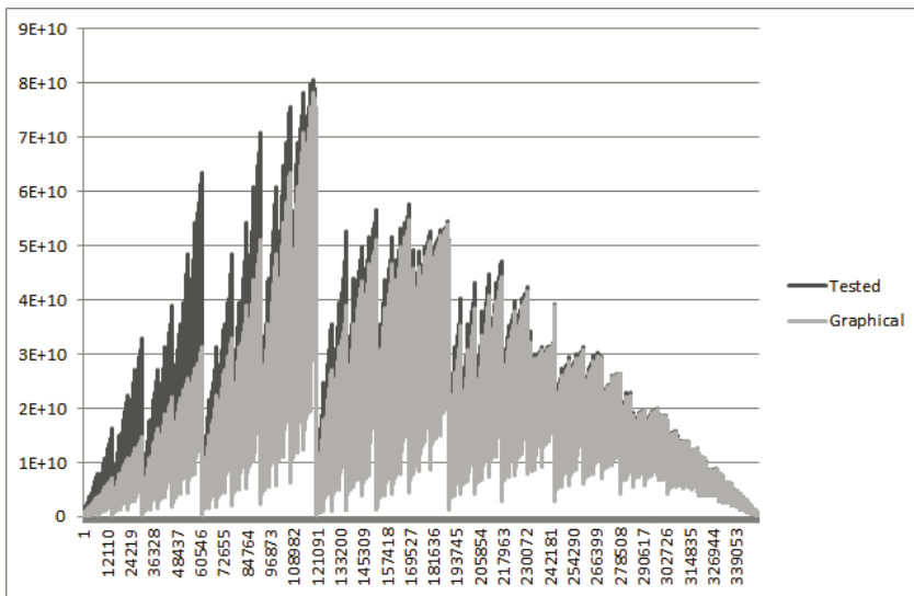
Figure 1: The number of tested (trimmed even) sequences and the number of graphical sequences as the function of the index of slices when n = 30
